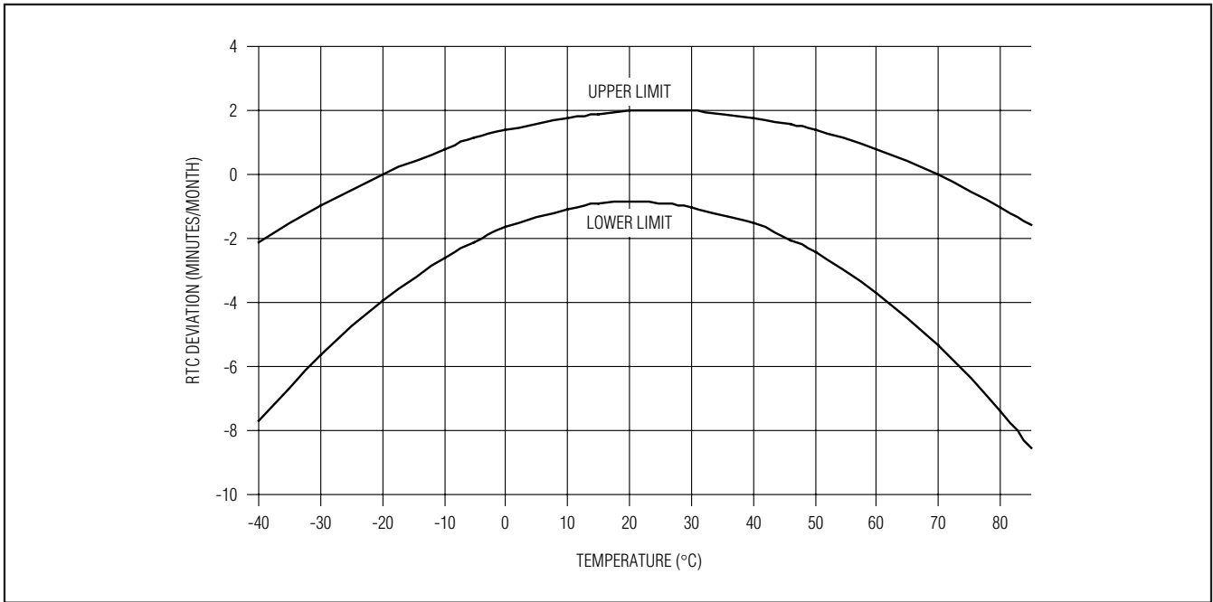
RTC Deviation vs. Temperature
